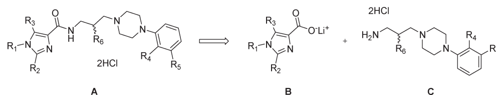
Figure 2. Preparation of target compounds using peptide bond formation.
