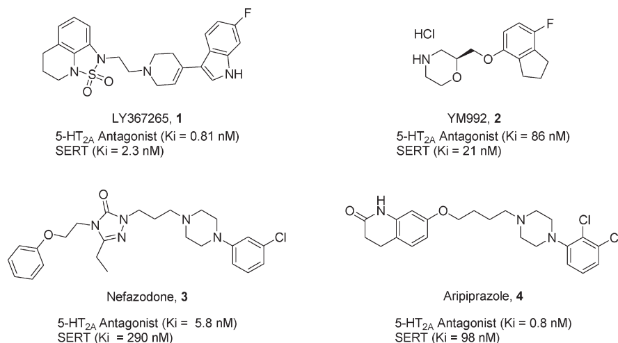
Figure 1. Chemical structures of representative antidepressant compounds.
